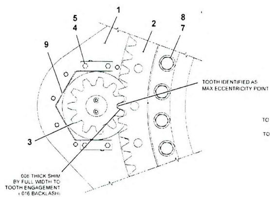
VIEW B-B
